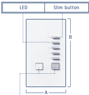
HWI-KP5 A = 2.75" (70.0mm) B = 4.50" (114.0mm)
