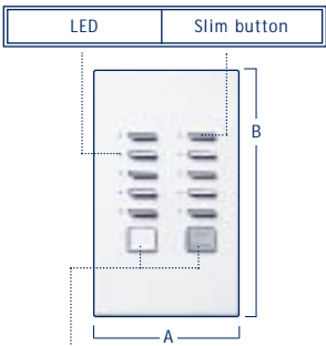
HWI-KP10 A = 2.75" (70.0mm) B = 4.50" (114.0mm)
