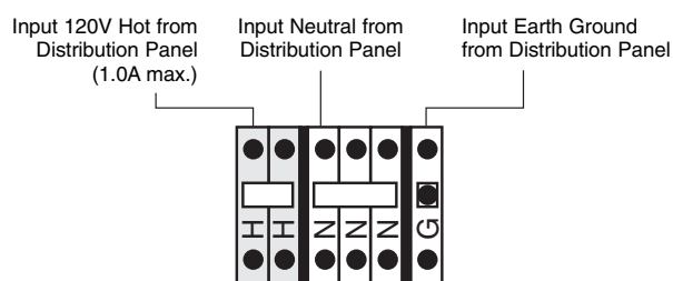
Figure 2 - Assembly Feed
