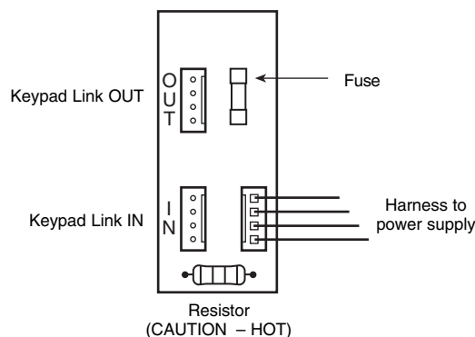
Figure 3 - Input/Output Board
