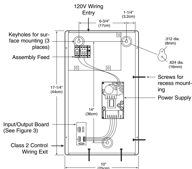
Figure 1 - HWI-PS
