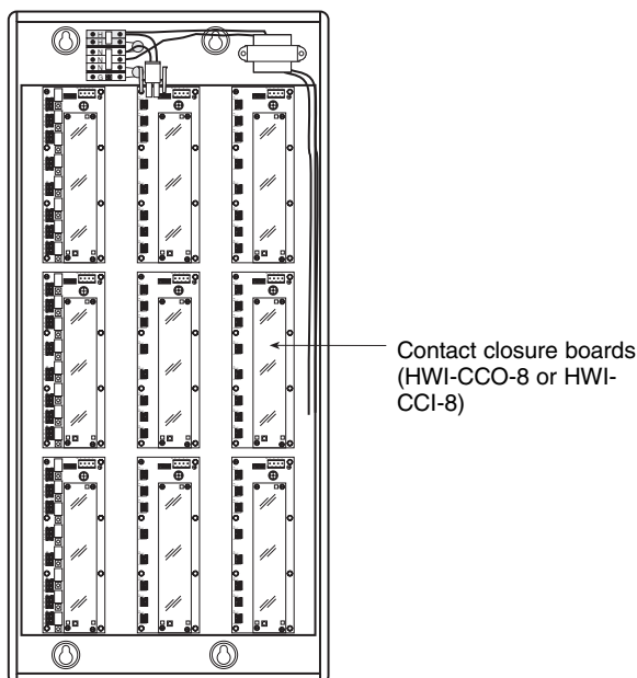
Figure 2 - Contact Closure Board Location
